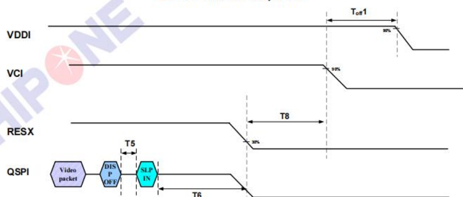
QSPI Power off sequence
